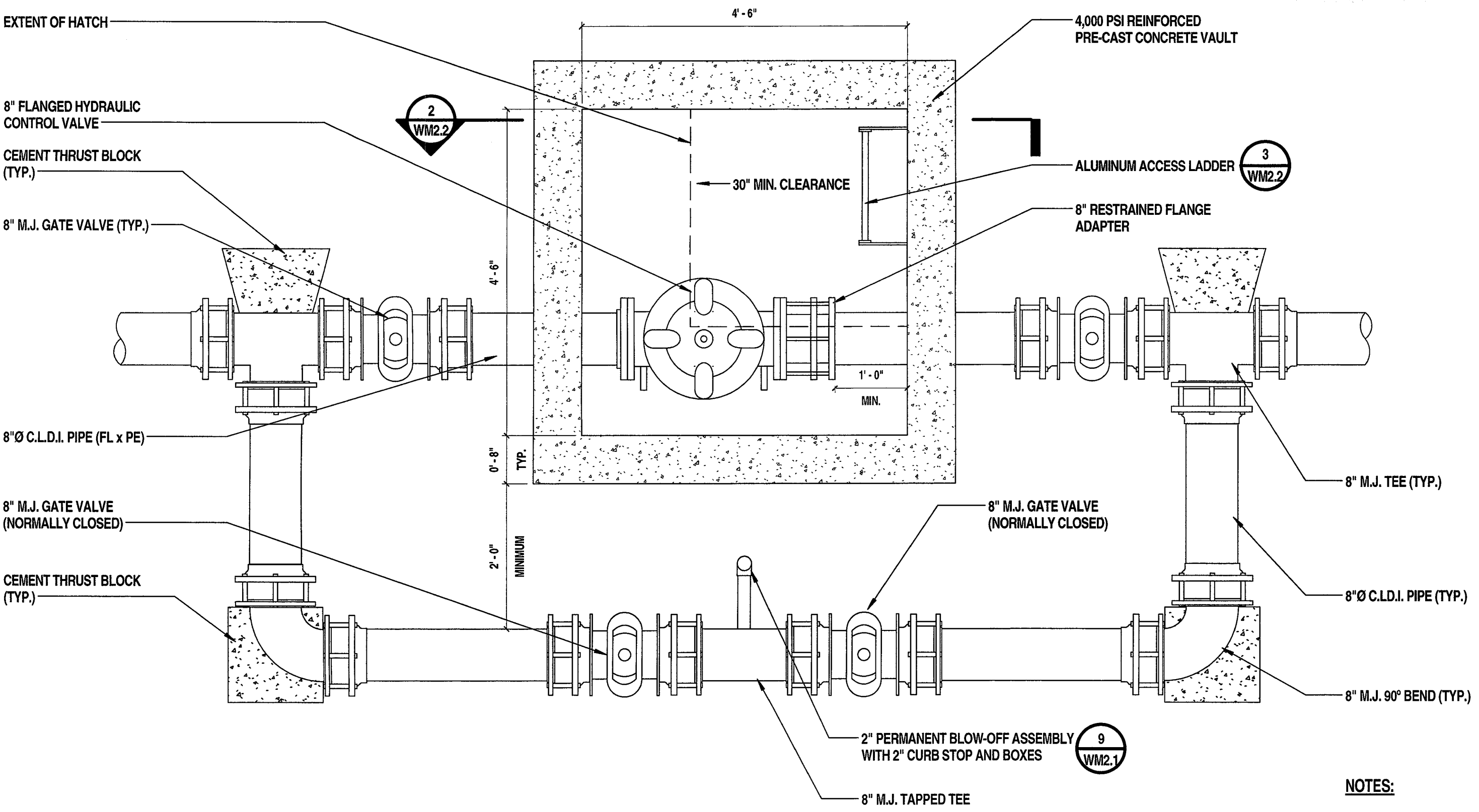
1 Control Valve Vault Plan
