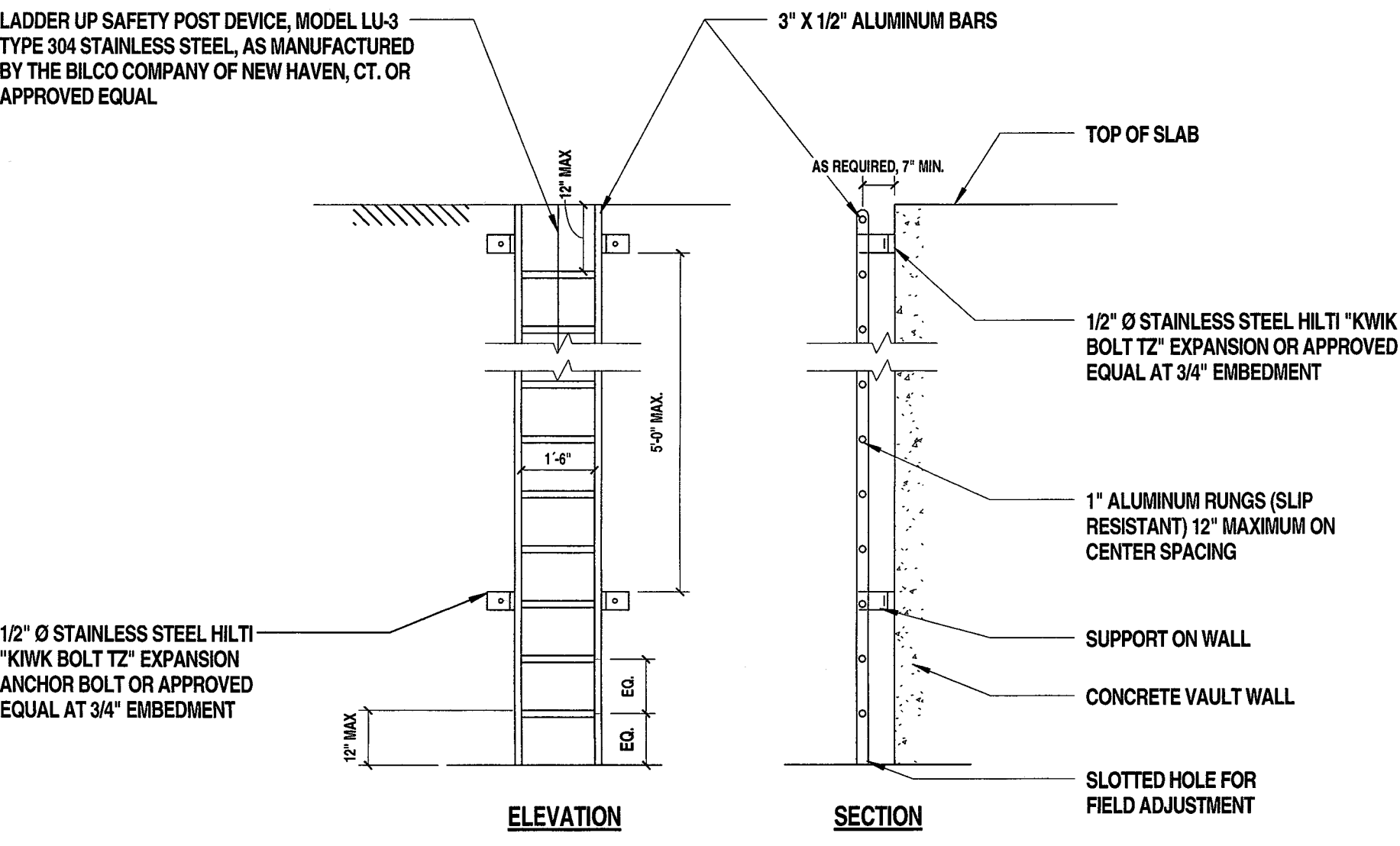
3 Access Ladder Detail
