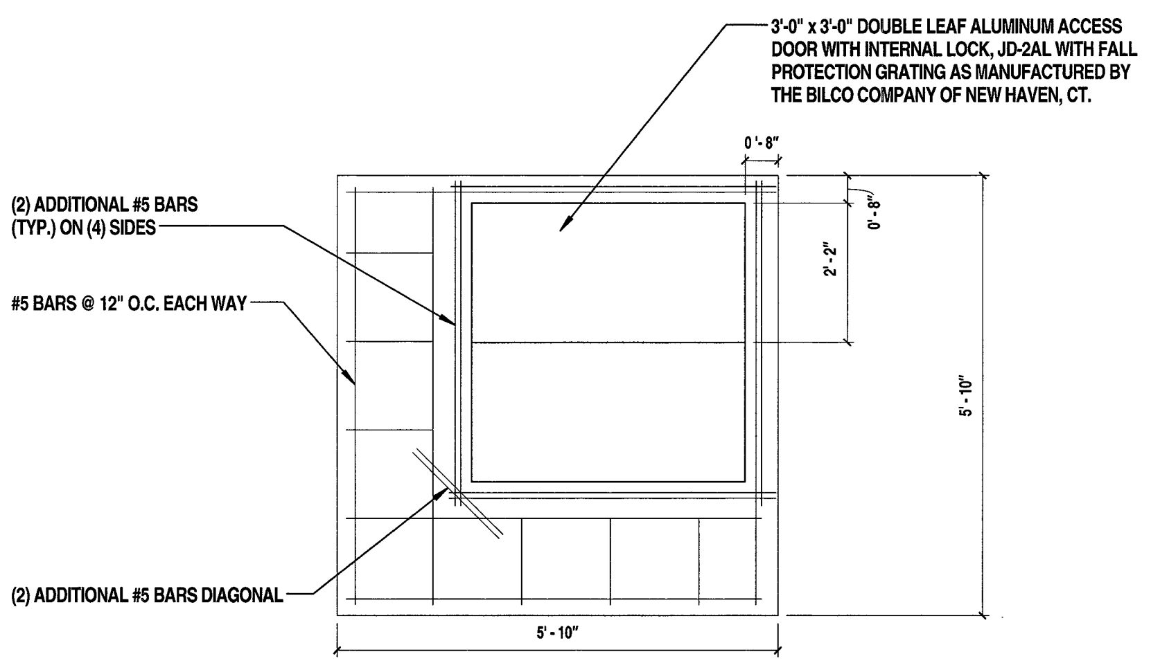
4 Vault Top Slab Detail
