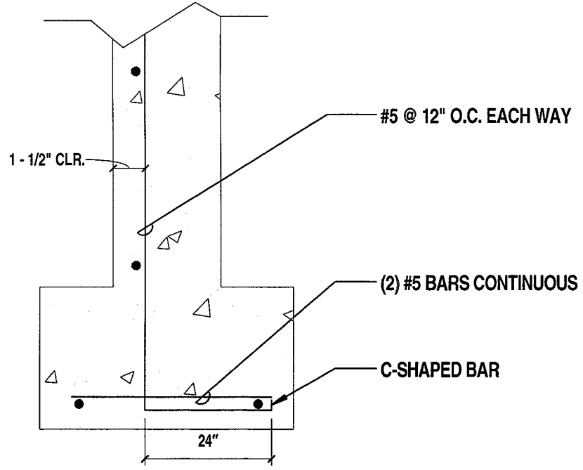
5 Typical Vault Wall Reinforcing Detail SCALE: NTS
