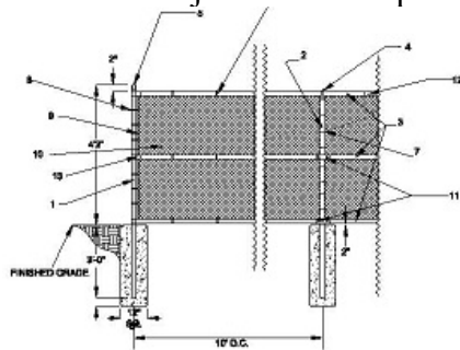
FENCE DETAIL
